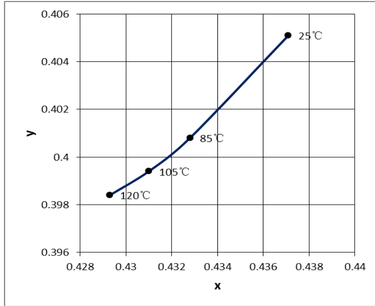
Fig 8. Chromaticity Coordinate vs. Junction Temperature, I_F=65mA (2600~4200K)
