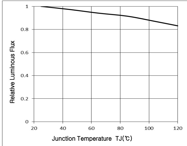
Fig 6. Junction Temperature vs. Relative Luminous Flux, I_F=65\text{mA}
