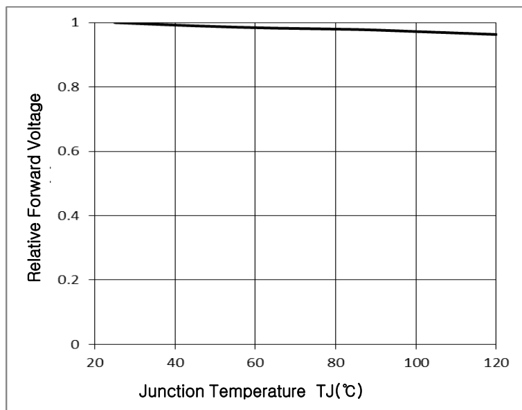
Fig 7. Junction Temperature vs. Relative Forward Voltage, I_F=65\text{mA}
